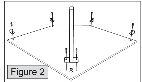
Brackets flush to edge
