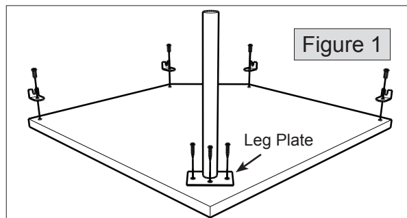
Brackets flush to edge
